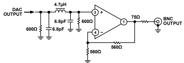
Figure 87. Example of Output Filter for ED, 8 \times Oversampling
