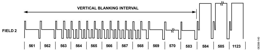
Figure 141. SMPTE 274M (1080i)
