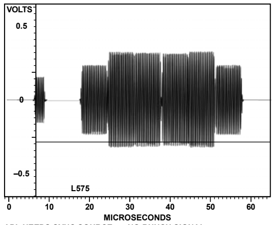
Figure 134. PAL Luma
