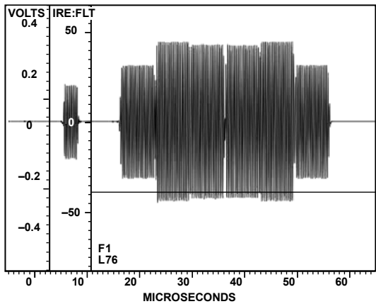
Figure 131. NTSC Luma
